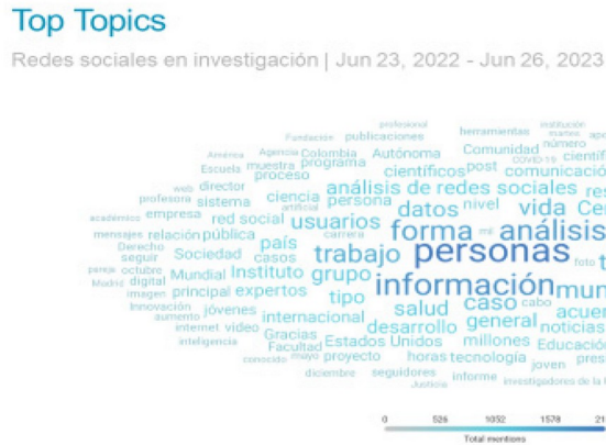
Figure 6. Top themes
